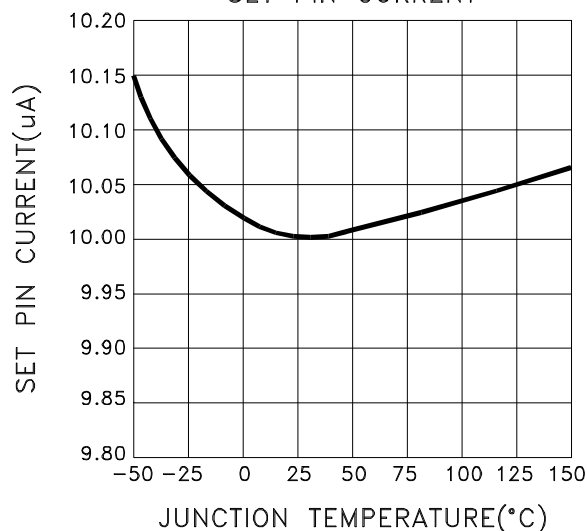
SET PIN CURRENT
