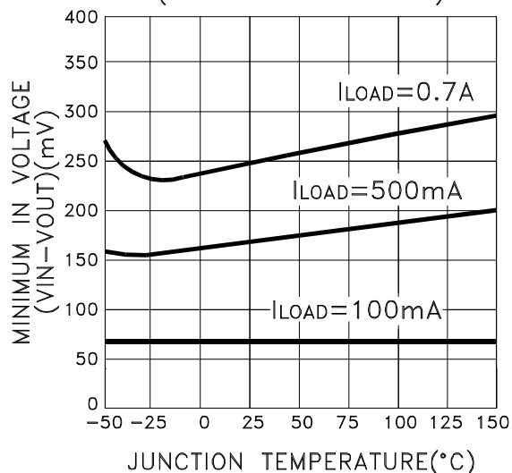
DROPOUT VOLTAGE (MINIMUM IN VOLTAGE)
